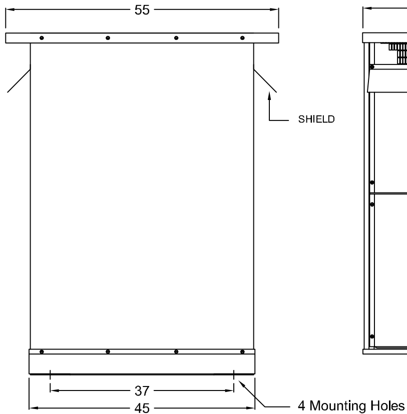
SIDE VIEW
